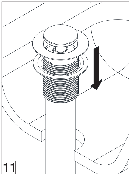
Drain installation
